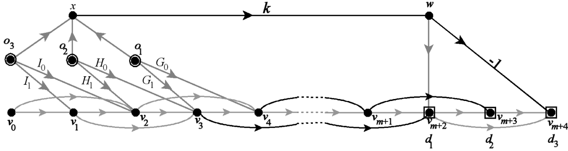
Figure 13: A more intuitive and more general digraph than Figure 12. The black arcs are required in all nonintersecting 3-routes.
