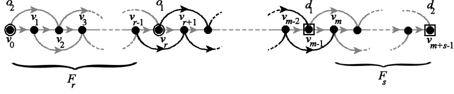
Figure 5: The directed graph associated with Cassini's generalized Fibonacci determinant, F_{m-r}F_{m+s} - F_mF_{m+s-r} = (-1)^{m+1-r} F_rF_s . The black arcs are required in a nonintersecting 2-route.
